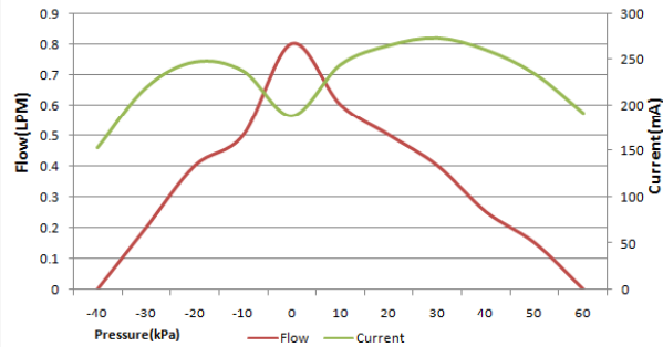
AJK-B03V1203 Flow(LPM) & Current(mA)
