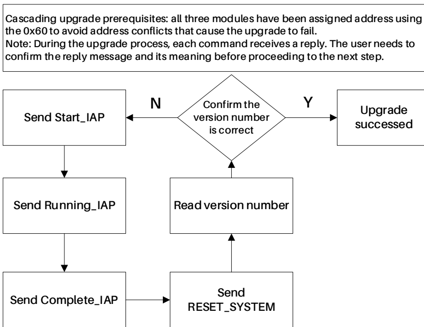
FIG 8 UPGRADE WORKFLOW
